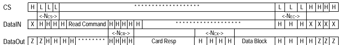
Figure 5-19. Timing diagram: Read CSD Register
