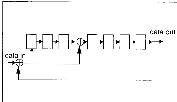
Figure 4-3. CRC7 Generator/Checker
