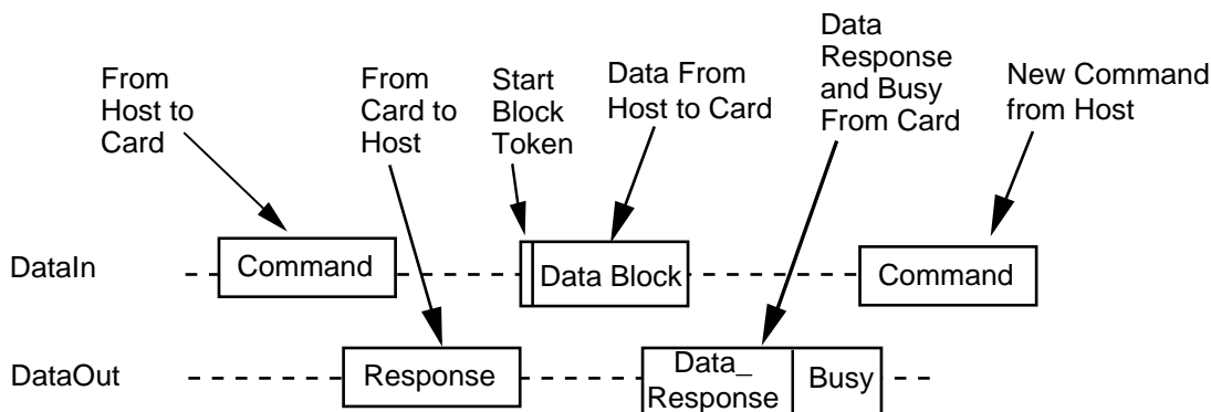
Figure 5-5. Single Block Write Operation
