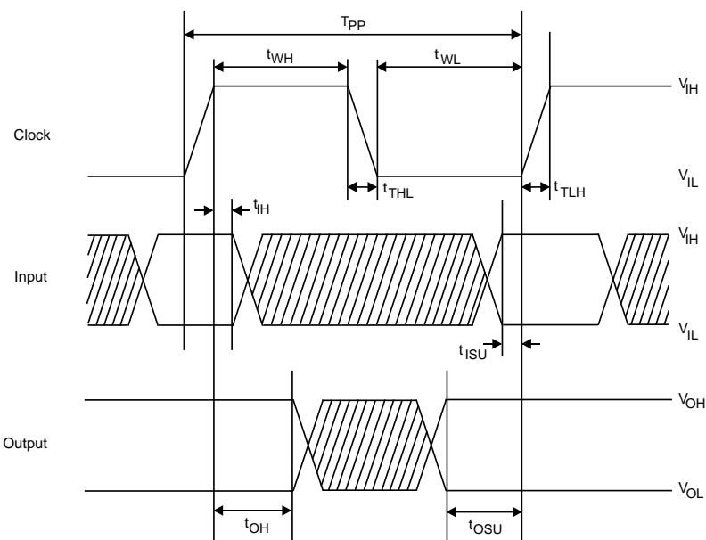
Figure 3-5. Timing Diagram Data Input/Output Referenced to Clock
