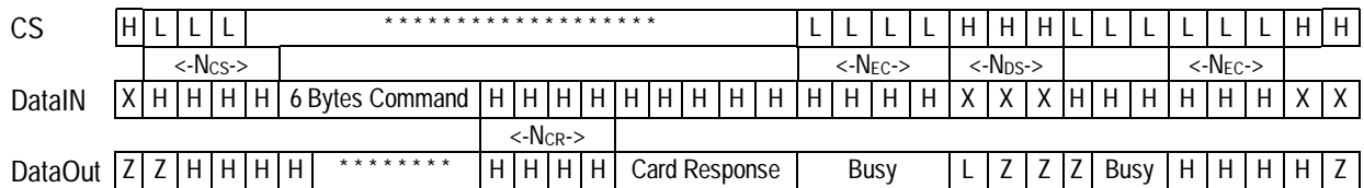
Figure 5-14. Timing Diagram of Command/Response Transaction, Card is Busy
