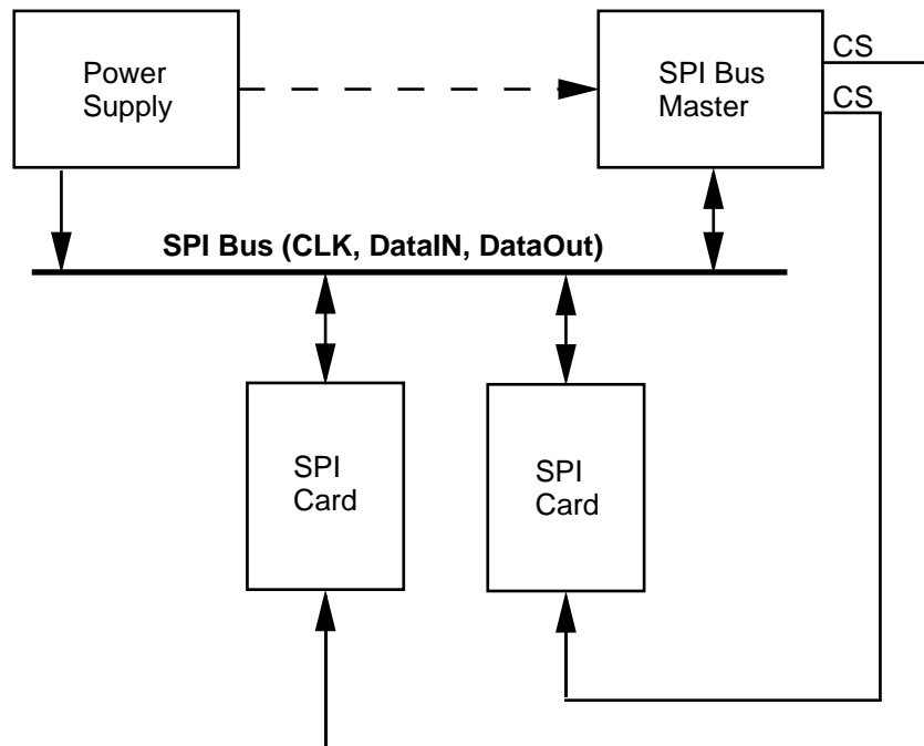
Figure 5-1. MultiMediaCard Bus System
