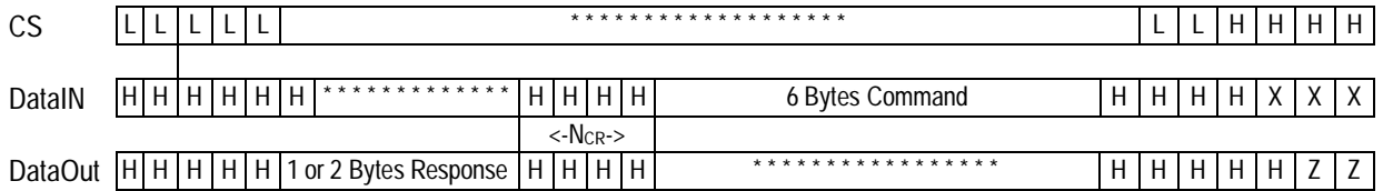
Figure 5-15. Timing Diagram: Card Response to the Next Host Command
