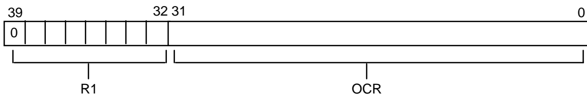
Figure 5-10. R3 Response Format
