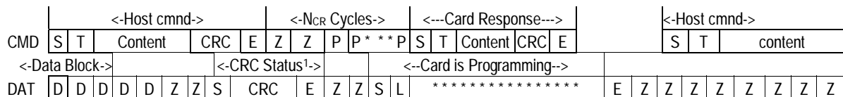
Figure 4-16. Stop Transmission During CRC Status Transfer from the Card
