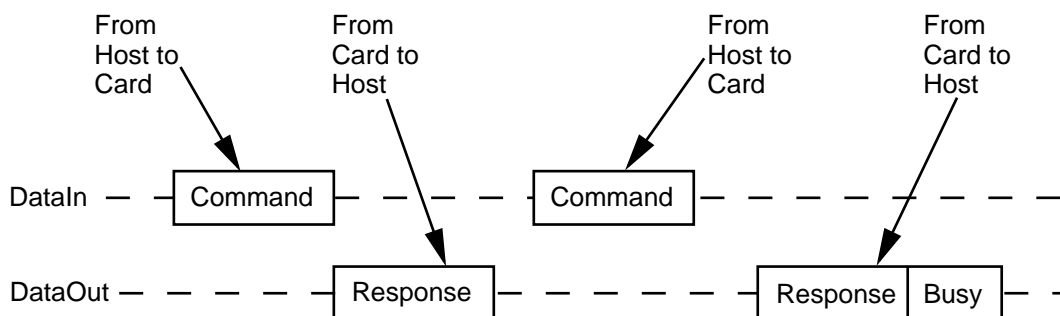
Figure 5-7. 'No data' Operations
