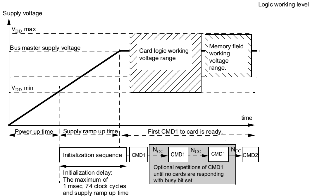
Figure 3-3. Power-up Diagram
