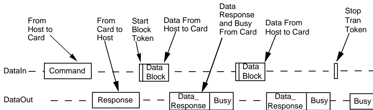
Figure 5-6. Multiple Block Write Operation
